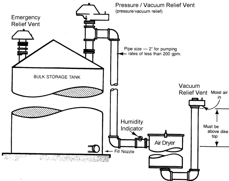
Image from Protectoseal. Series 782 air dryer. https://www.protectoseal.com/specialty-valves-and-fittings/
